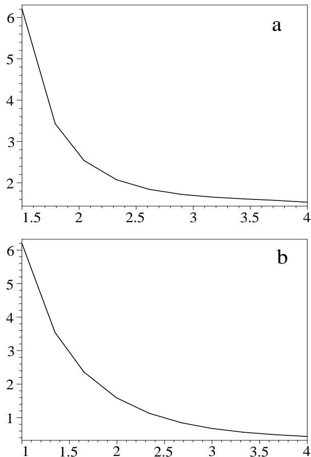
FIG. 4: Variation of the critical value \beta_c for the onset of filamentation instability versus the equilibrium electron temperature anisotropy a_e for a_p = 1 , \tau_e = 1 , X = 0 (panel a) and versus the ratio of the electron to proton equilibrium parallel temperature \tau_e for a_p = 1 , a_e = 1.5 , X = 0 (panel b).
