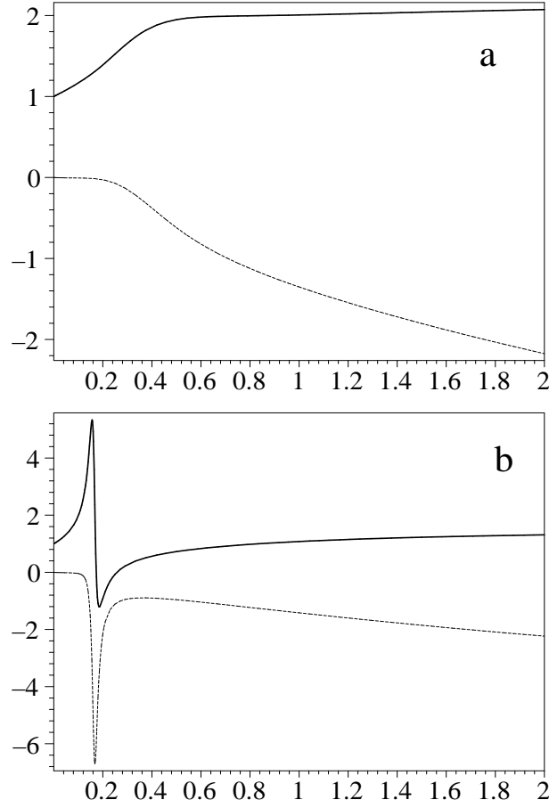
FIG. 1: Variations of \chi_* (solid line) and \nu_* (dashed line) as a function of \beta_{\parallel p} for an equilibrium state with isotropic ion and electron temperatures ( a_p = 1 , a_e = 1 ), and no alpha-particles ( X = 0 ). In panel (a), ions and electrons have the same equilibrium temperature ( \tau_e = 1 ), while in panel (b), the ratio of the electron temperature to that of the protons is \tau_e = 8 . Negative values for \chi_* imply filamentation instability.
