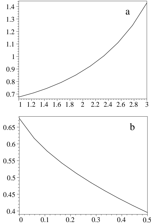
FIG. 5: Variation of \beta_c as a function of the anisotropy degree of the proton equilibrium temperature a_p for a_e = 1.5 , \tau_e = 3 , X = 0 (panel a) and as a function of the relative alpha-particle number density, measured by X for a_p = 1 , \tau_e = 3 , a_e = 1.5 (panel b).
