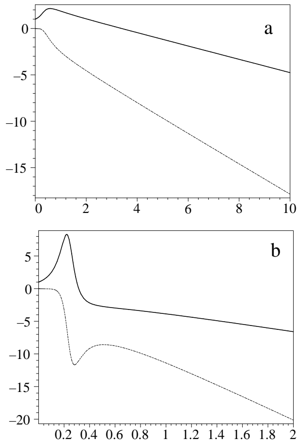
FIG. 3: Same as Fig. 1 with, in panel (a), a_p = 1 , \tau_e = 1 , X = 0 , and a_e = 1.8 (corresponding to isotropic proton and anisotropic electron equilibrium temperatures), and in panel (b) a_p = 3.25 , a_e = 1.27 , a_\alpha = 3.25 , \tau_e = 5.5 , \tau_\alpha = 4 , X = 0.1 , \mu_\alpha = 4 and Z = 2 (corresponding to anisotropic temperatures for all species, with hotter electrons and alpha-particles whose number density is 10% that of the protons).
